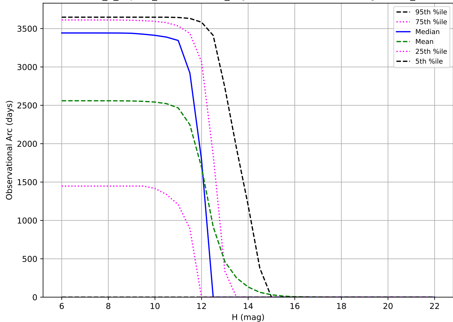
uniform_u_expt38_nscale1.1v3.4_10yrs: Observational Arc Length OCC_r20
