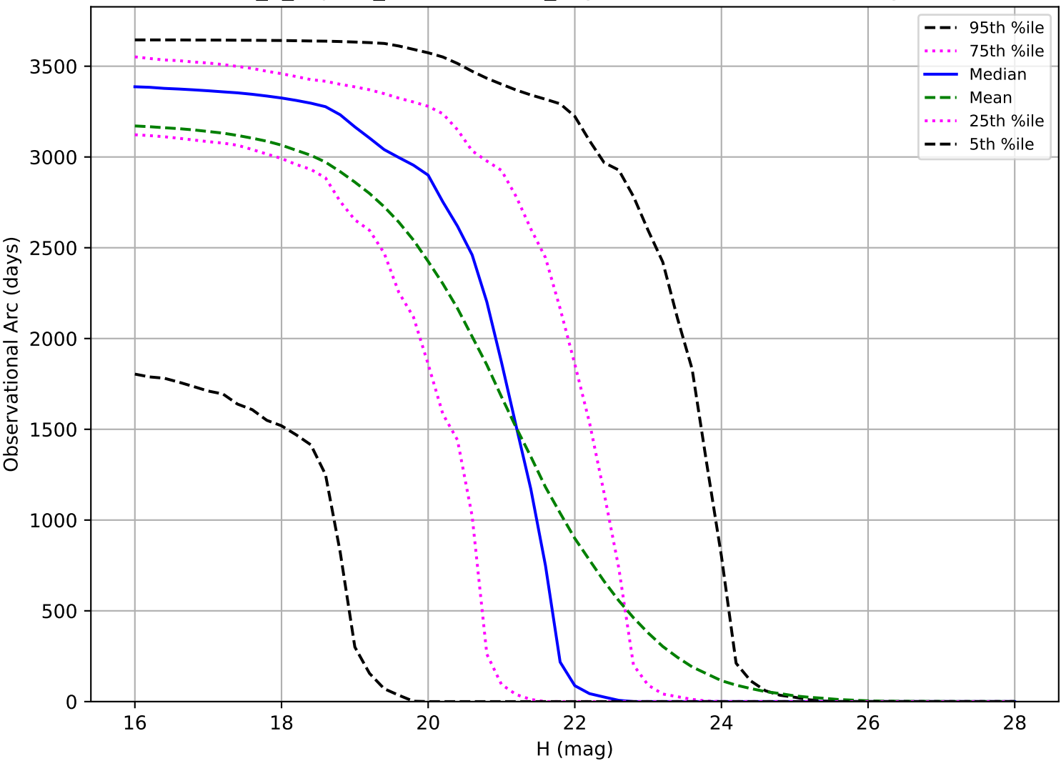
uniform_u_expt38_nscale1.1v3.4_10yrs: Observational Arc Length NEO
