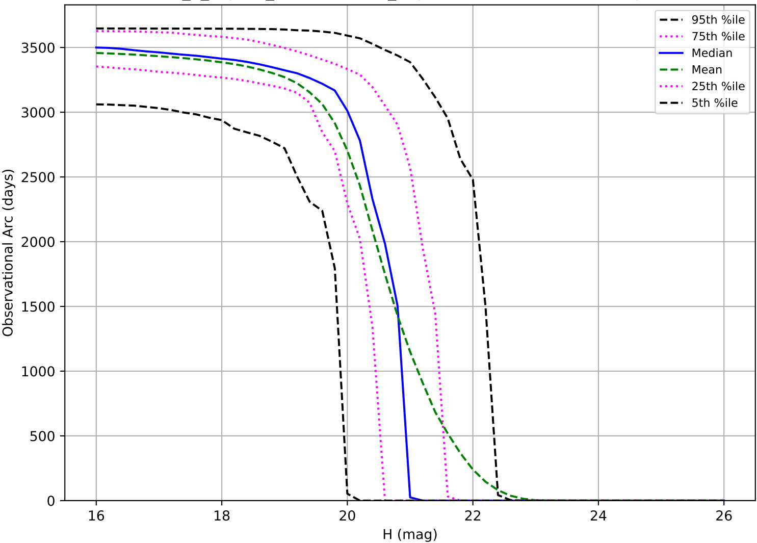
uniform_u_expt38_nscale1.1v3.4_10yrs: Observational Arc Length MBA
