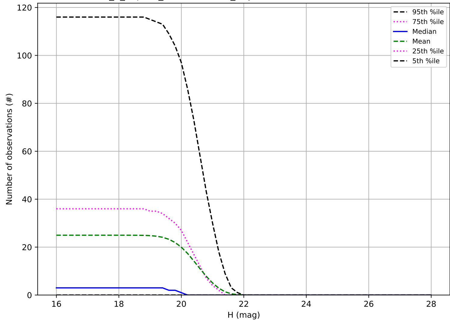
uniform_u_expt38_nscale1.1v3.4_10yrs: Number of observations Vatira
