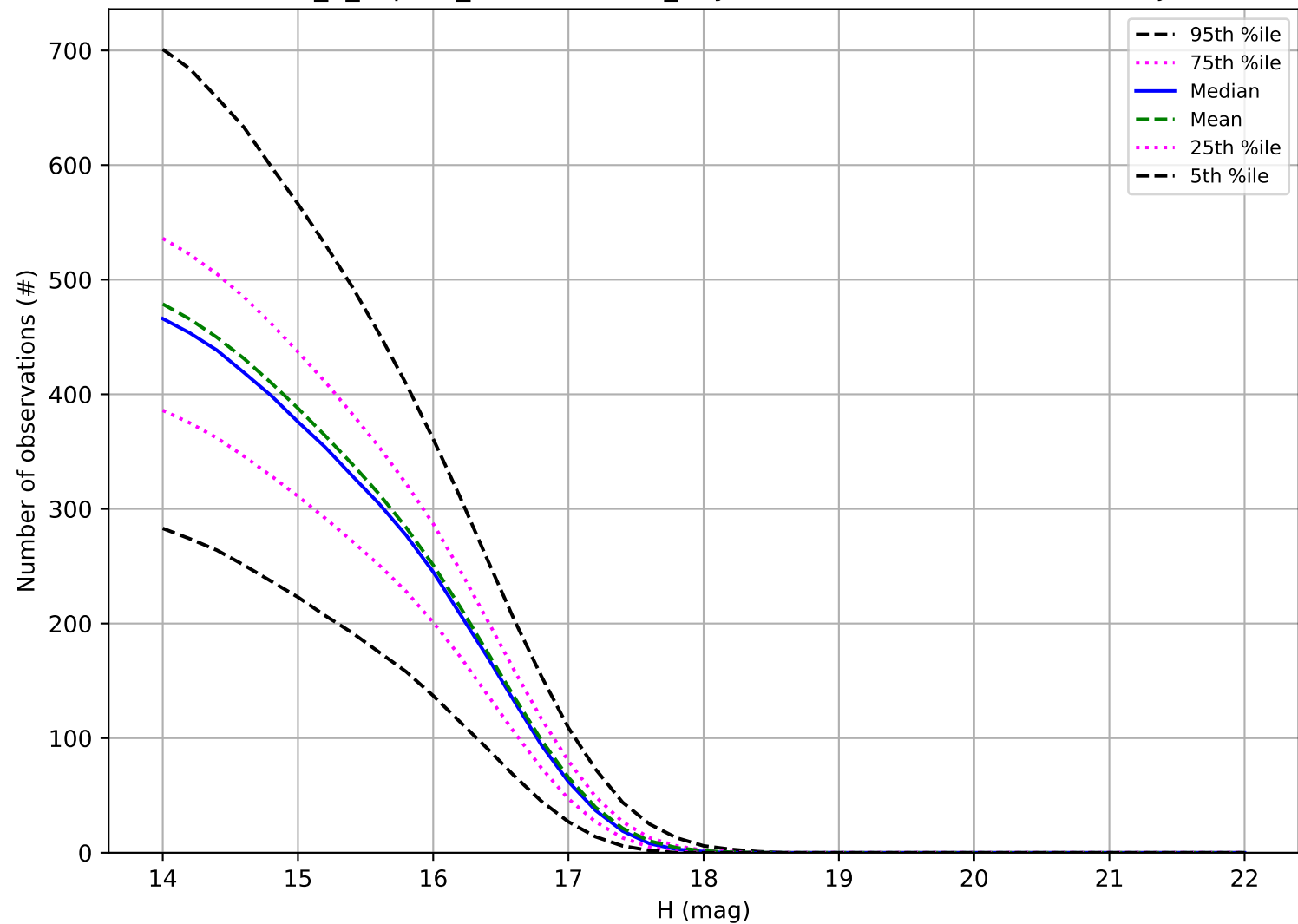
uniform_u_expt38_nscale1.1v3.4_10yrs: Number of observations Trojan
