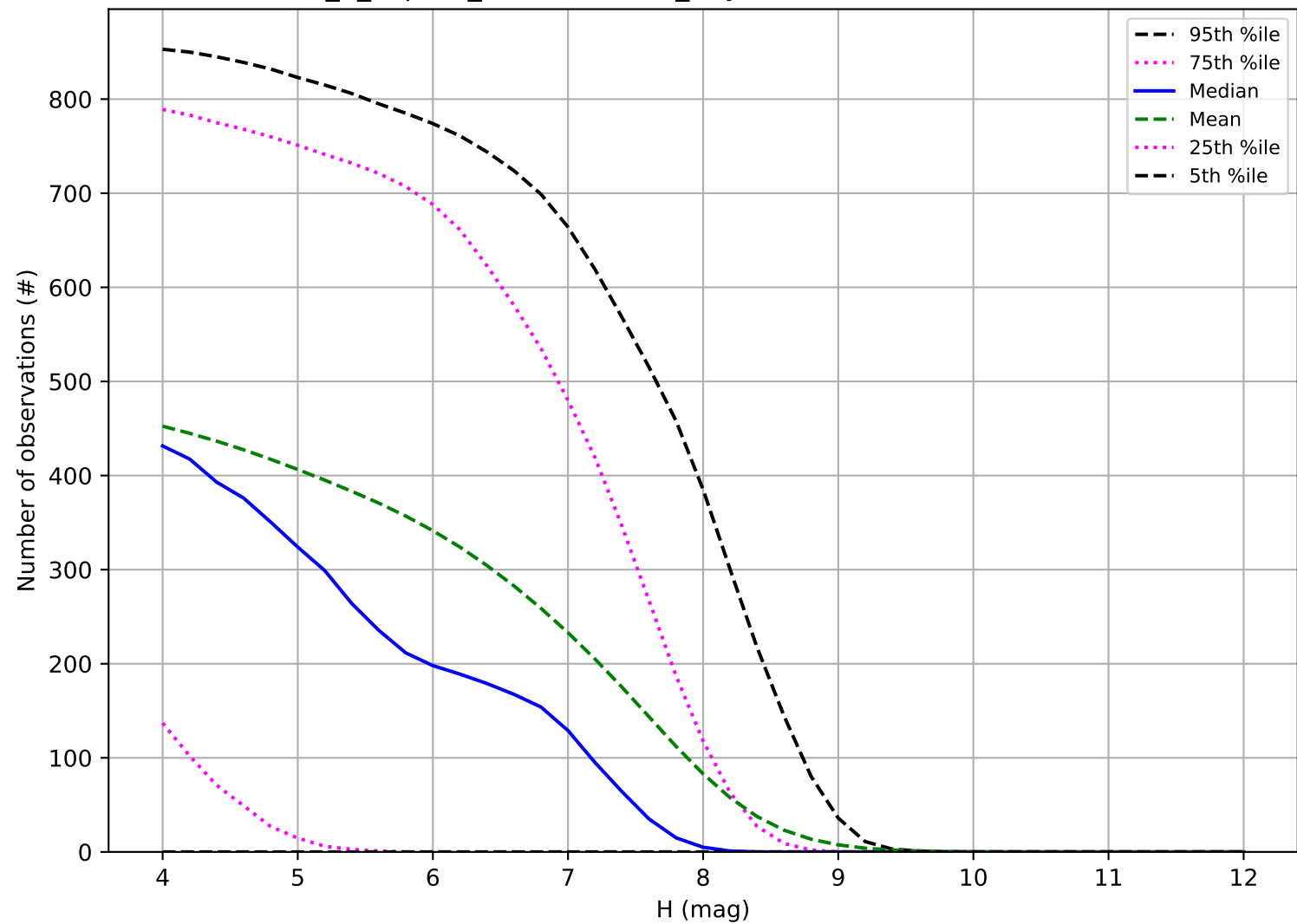
uniform_u_expt38_nscale1.1v3.4_10yrs: Number of observations TNO
