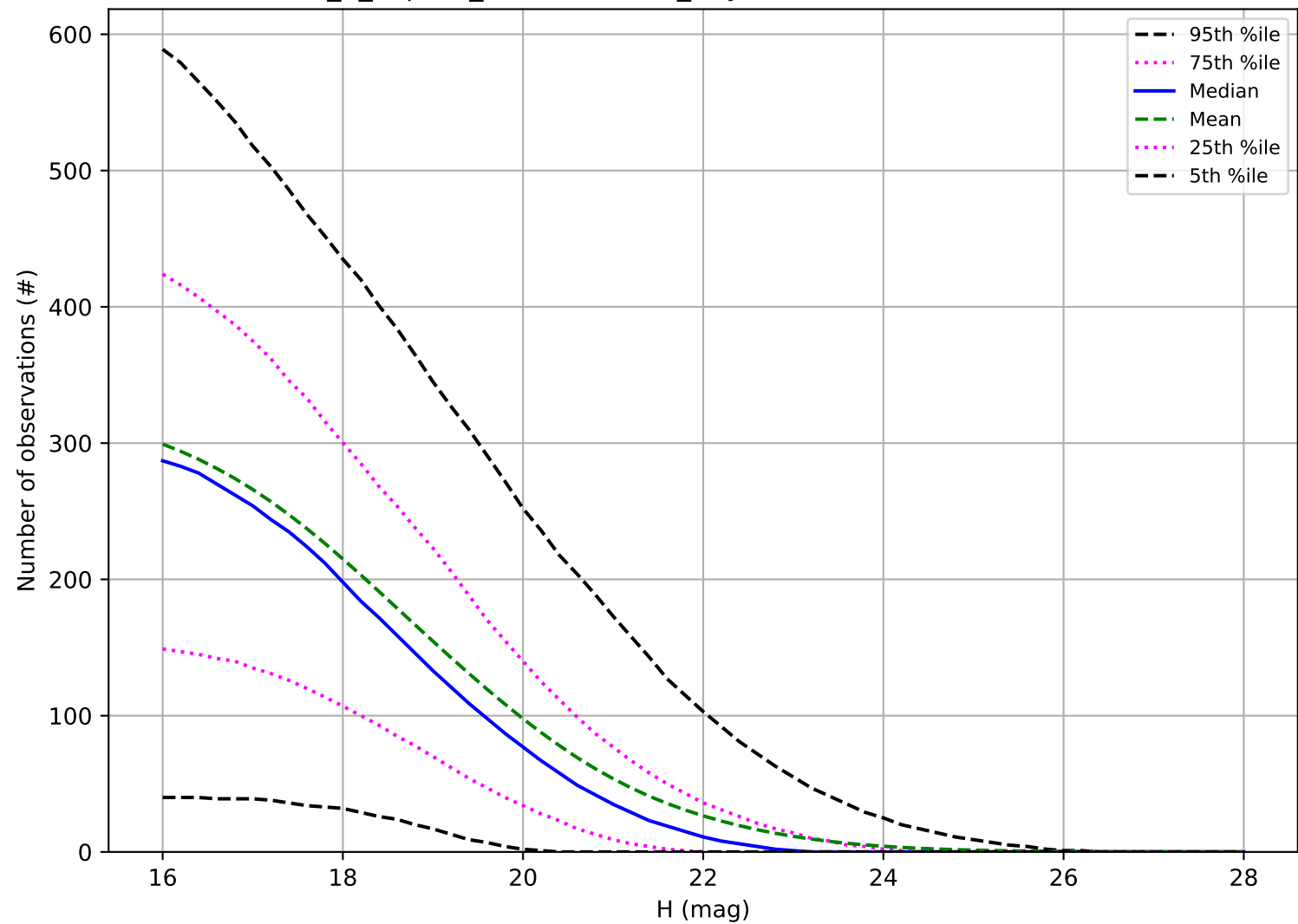
uniform_u_expt38_nscale1.1v3.4_10yrs: Number of observations PHA
