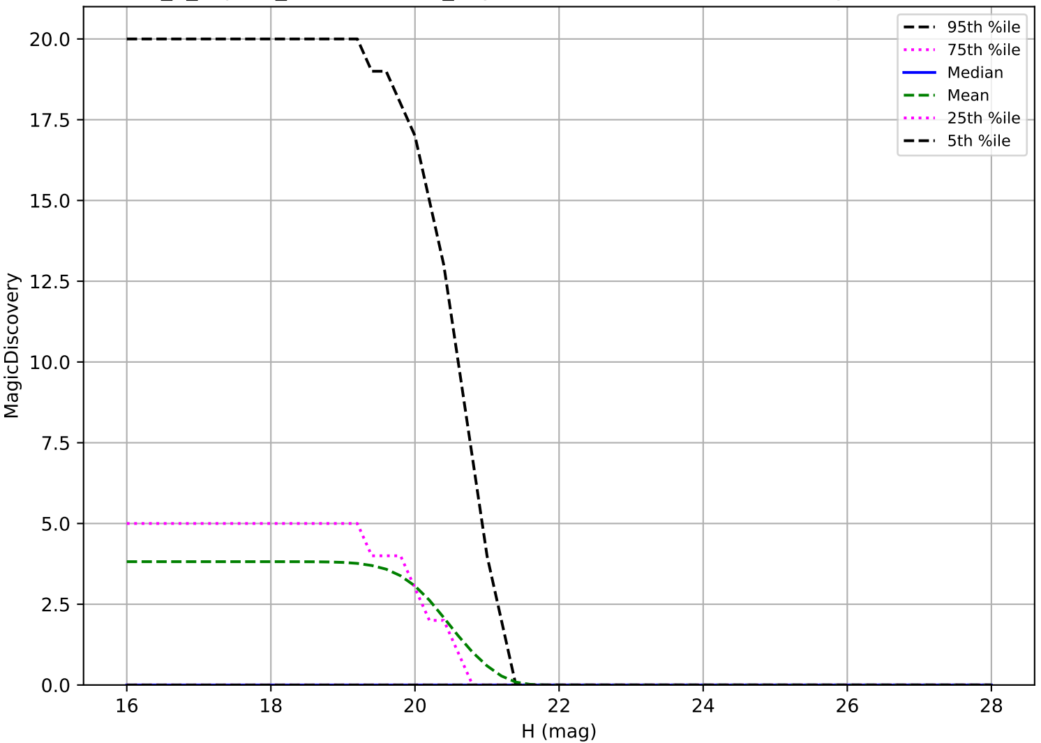
uniform_u_expt38_nscale1.1v3.4_10yrs: Vatira 6 detections in 60 nights detection loss
