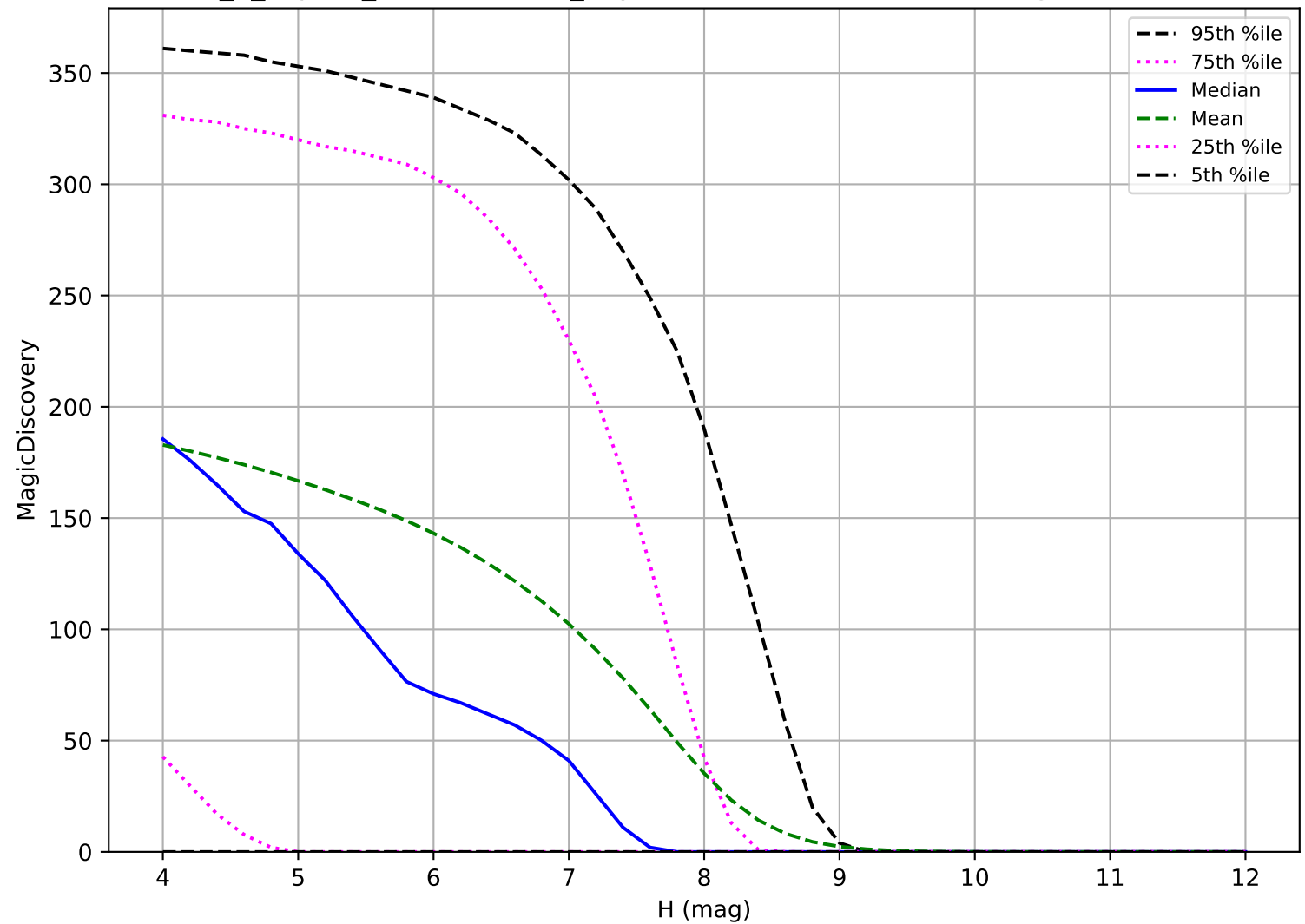
uniform_u_expt38_nscale1.1v3.4_10yrs: TNO 6 detections in 60 nights detection loss
