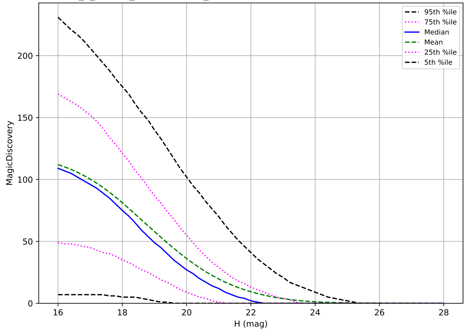
uniform_u_expt38_nscale1.1v3.4_10yrs: PHA 6 detections in 60 nights detection loss
