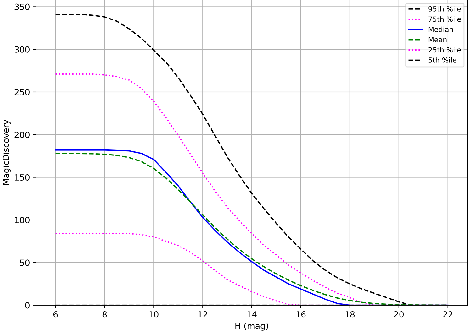
uniform_u_expt38_nscale1.1v3.4_10yrs: OCC_r5 6 detections in 60 nights detection loss
