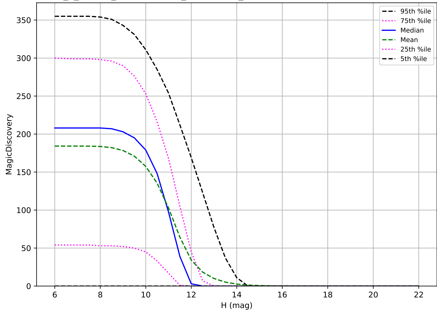
uniform_u_expt38_nscale1.1v3.4_10yrs: OCC_r20 6 detections in 60 nights detection loss
