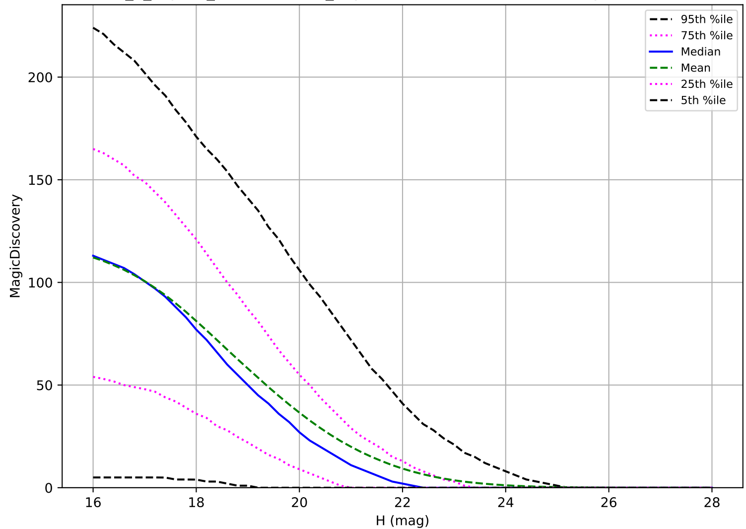
uniform_u_expt38_nscale1.1v3.4_10yrs: NEO 6 detections in 60 nights detection loss
