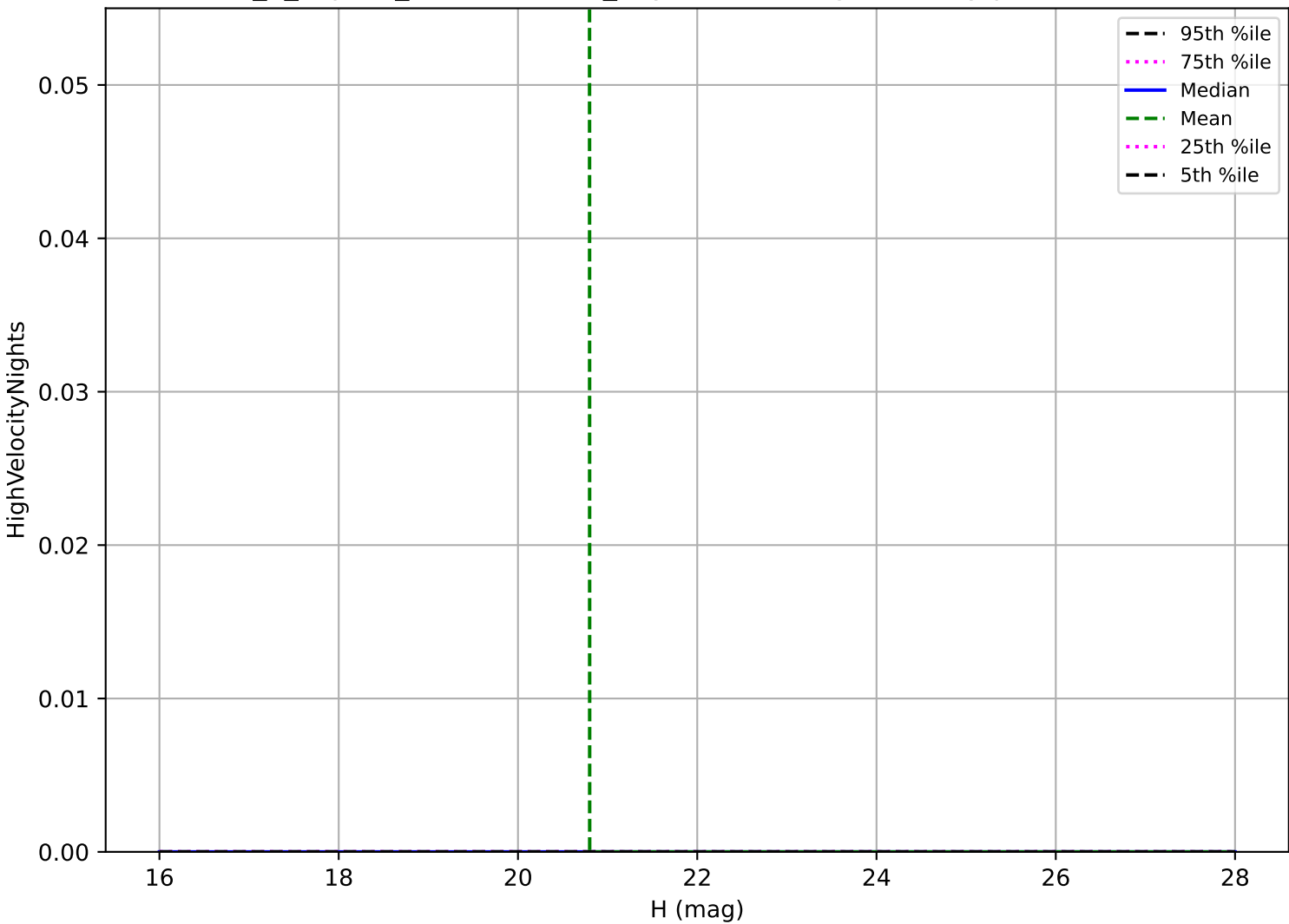
uniform_u_expt38_nscale1.1v3.4_10yrs: Vatira High velocity pair detection loss
