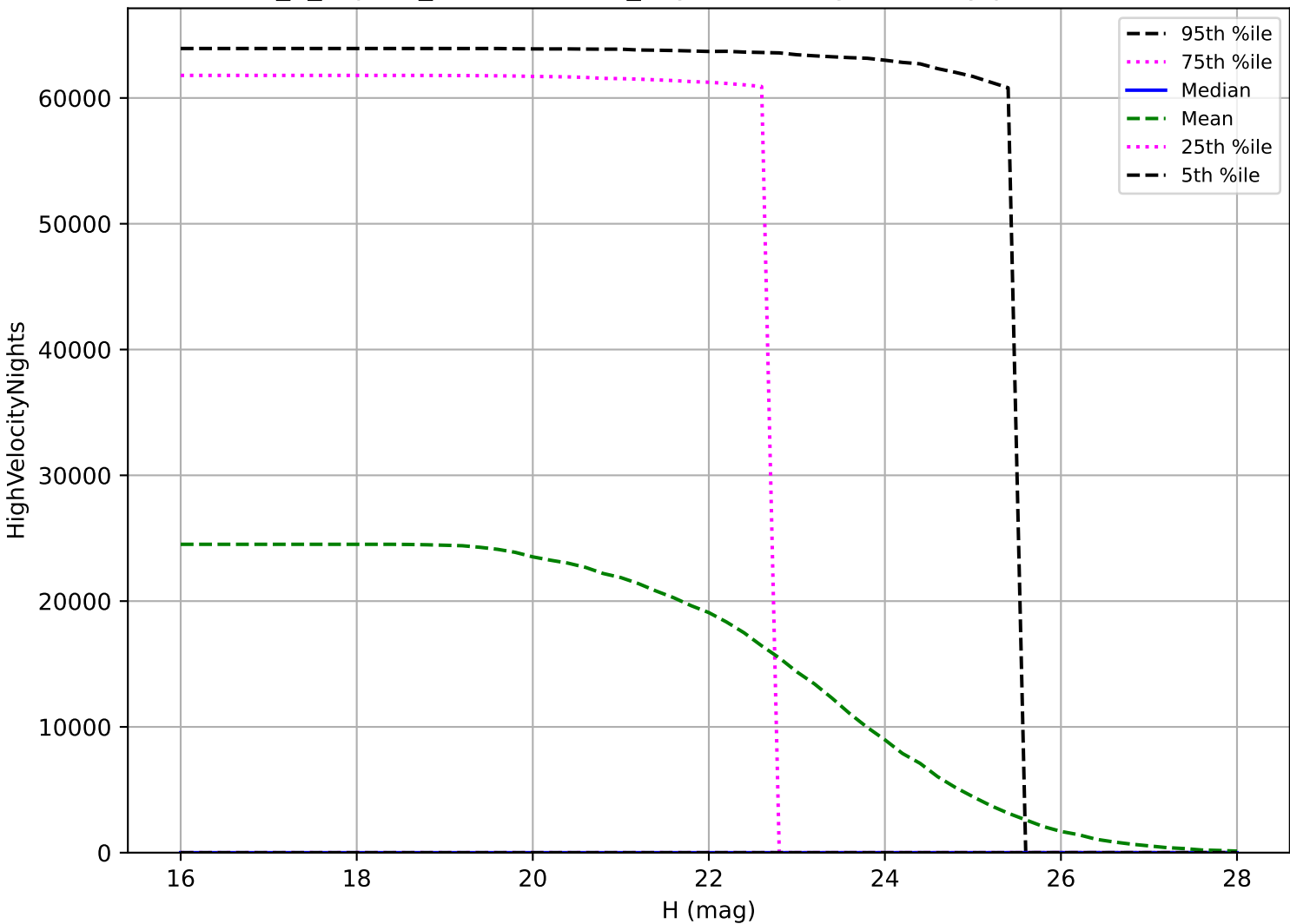
uniform_u_expt38_nscale1.1v3.4_10yrs: PHA High velocity pair detection loss
