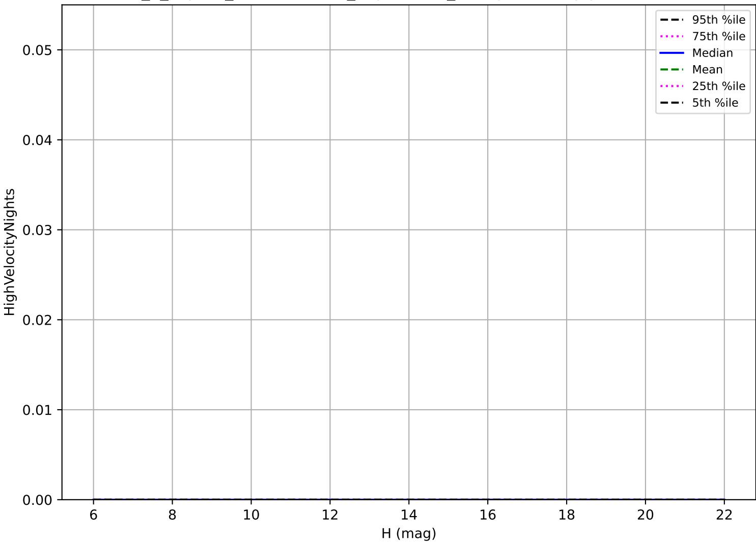
uniform_u_expt38_nscale1.1v3.4_10yrs: OCC_r5 High velocity pair detection loss
