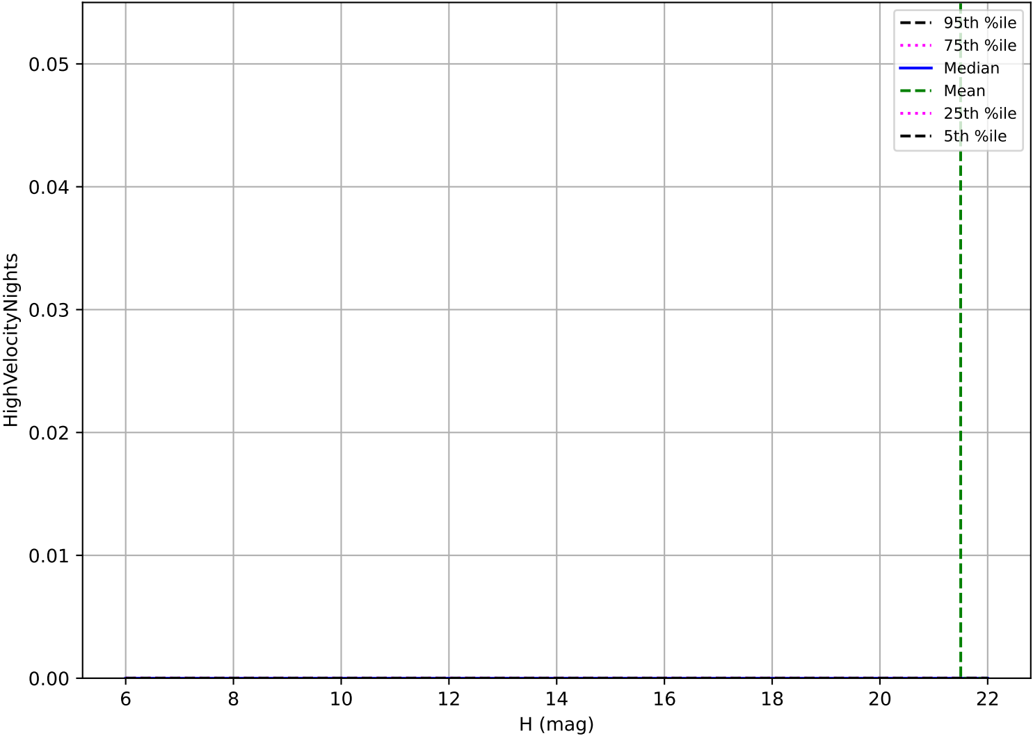
uniform_u_expt38_nscale1.1v3.4_10yrs: OCC_r20 High velocity pair detection loss
