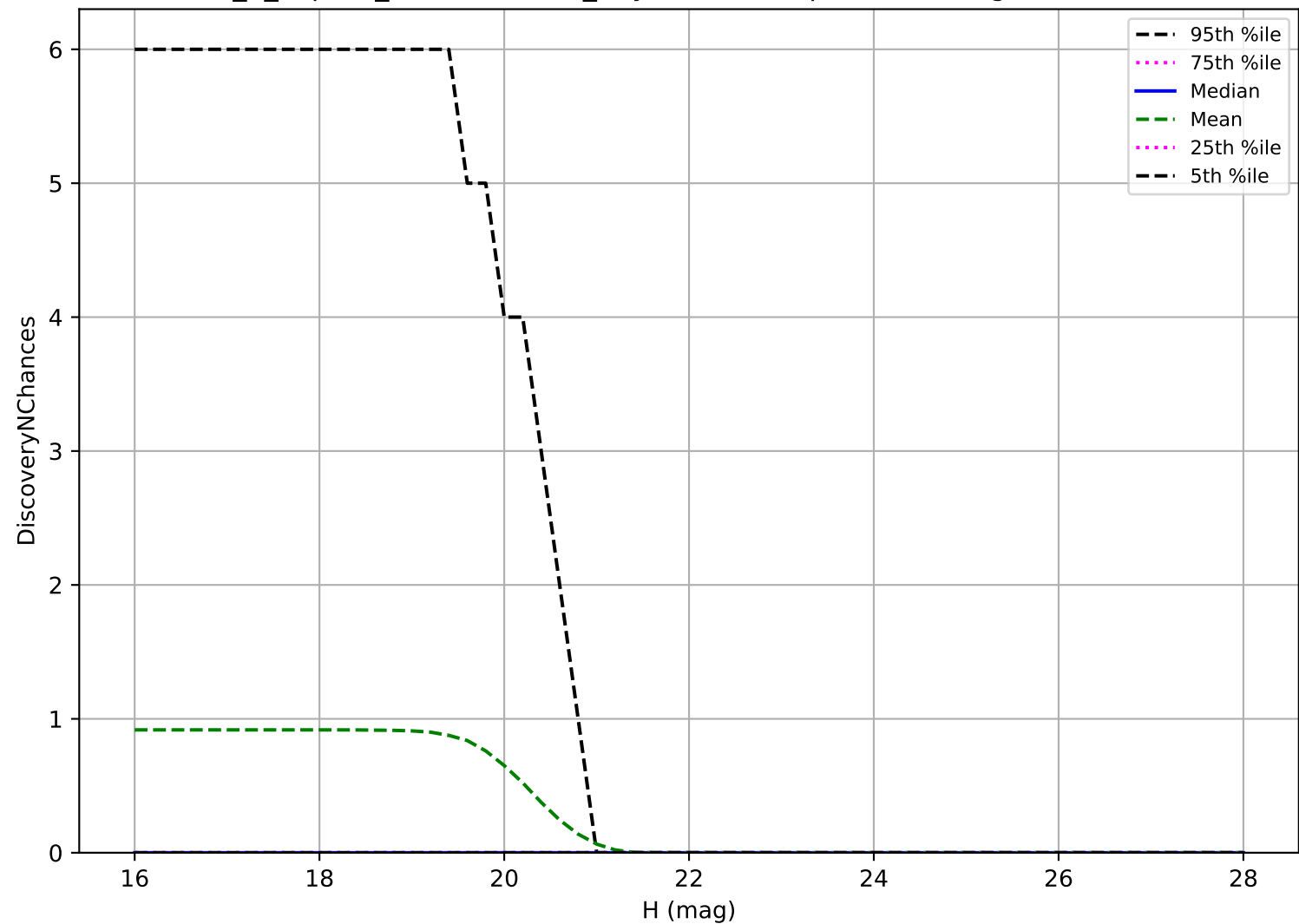
uniform_u_expt38_nscale1.1v3.4_10yrs: Vatira 3 pairs in 15 nights detection loss
