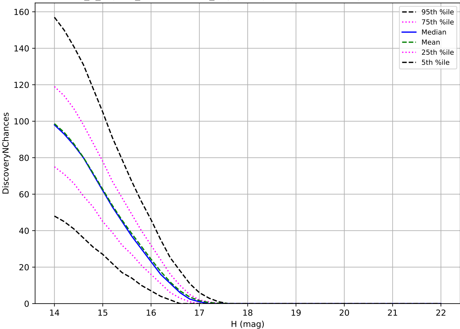
uniform_u_expt38_nscale1.1v3.4_10yrs: Trojan 3 pairs in 15 nights detection loss
