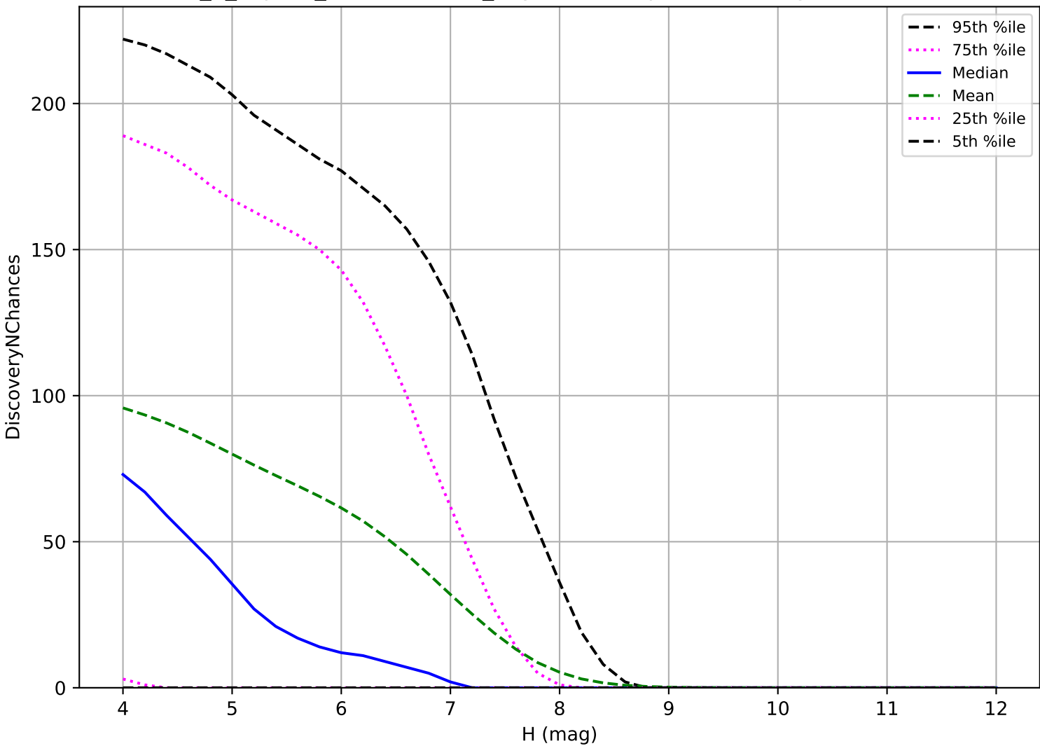
uniform_u_expt38_nscale1.1v3.4_10yrs: TNO 3 pairs in 15 nights detection loss
