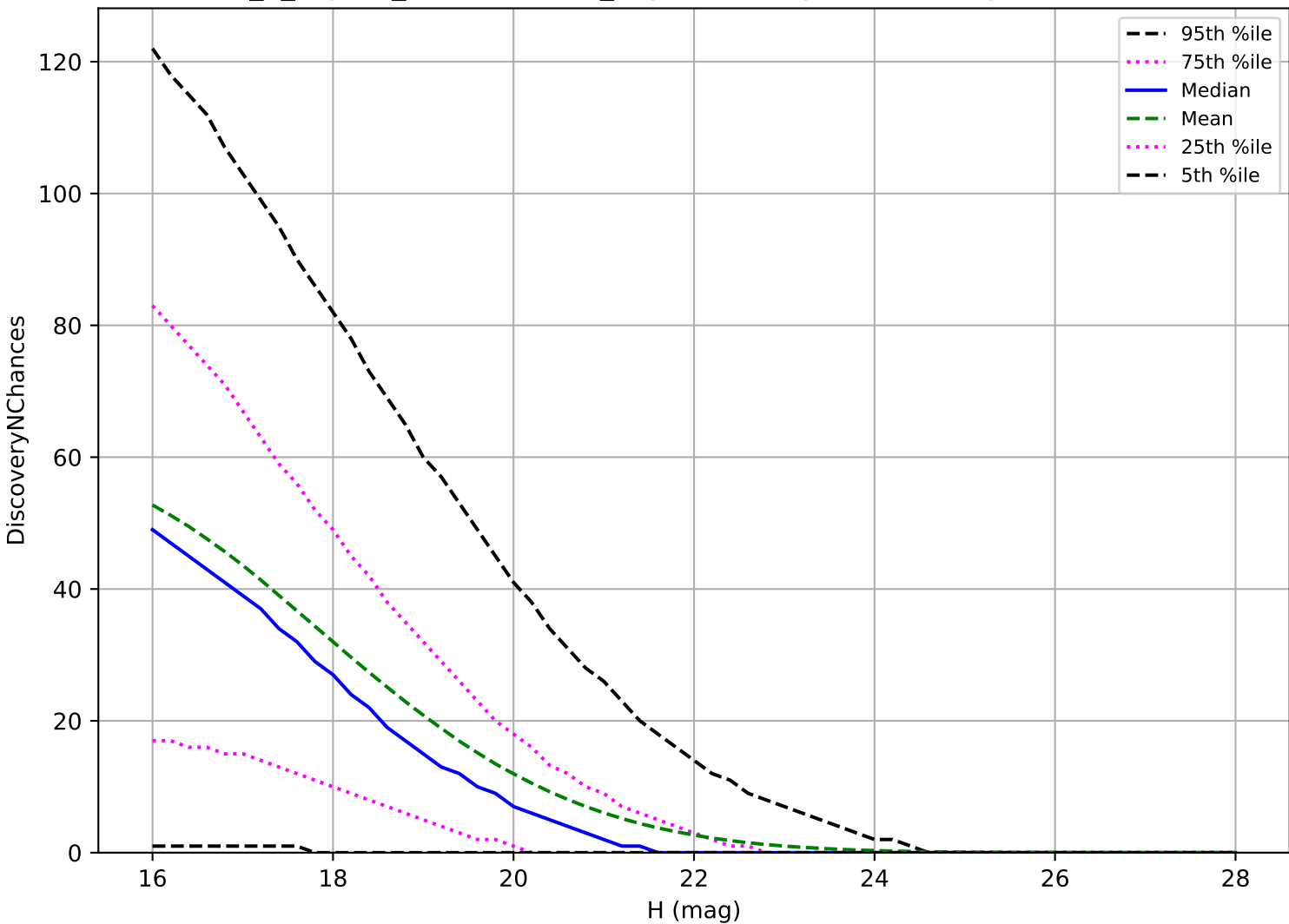
uniform_u_expt38_nscale1.1v3.4_10yrs: PHA 3 pairs in 15 nights detection loss
