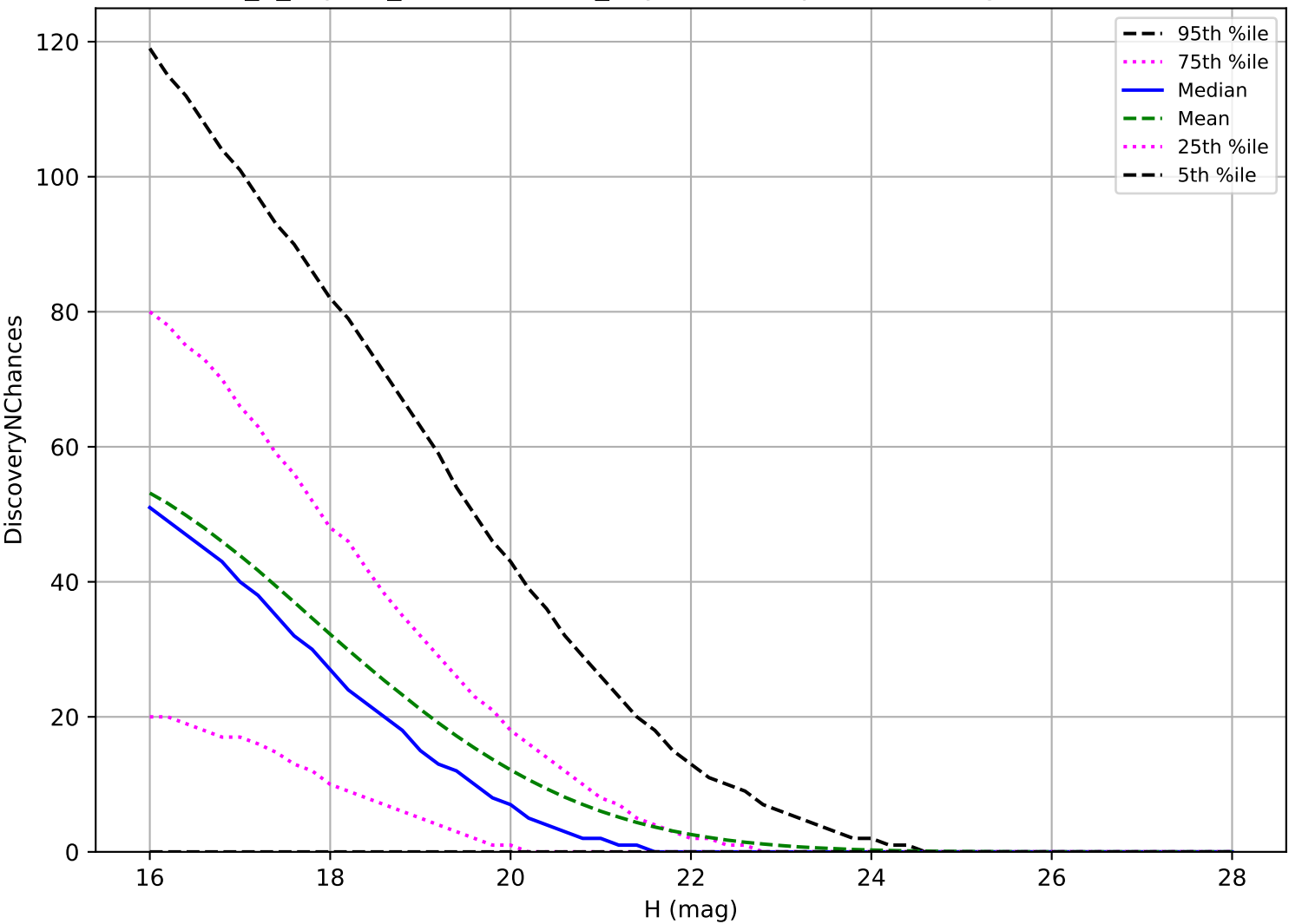
uniform_u_expt38_nscale1.1v3.4_10yrs: NEO 3 pairs in 15 nights detection loss
