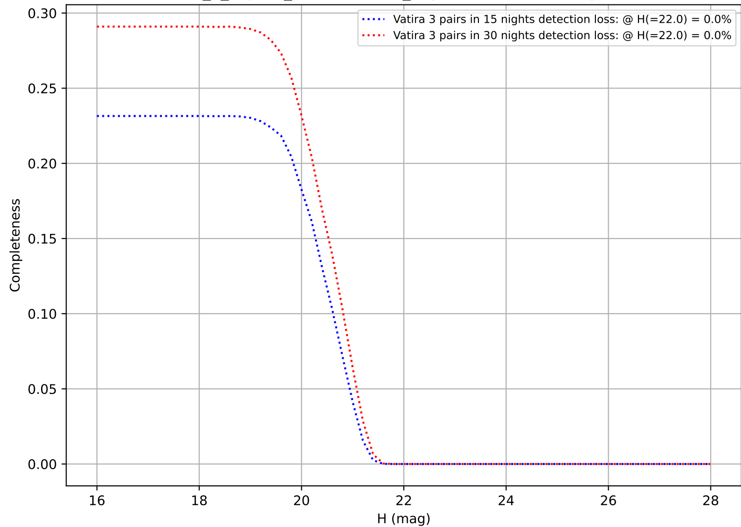
uniform_u_expt38_nscale1.1v3.4_10yrs: DifferentialCompleteness
