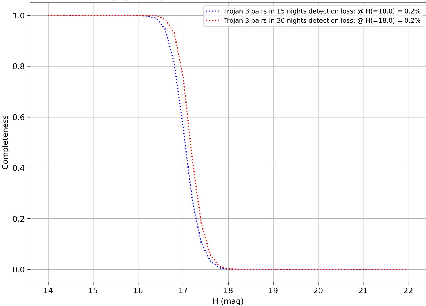
uniform_u_expt38_nscale1.1v3.4_10yrs: DifferentialCompleteness
