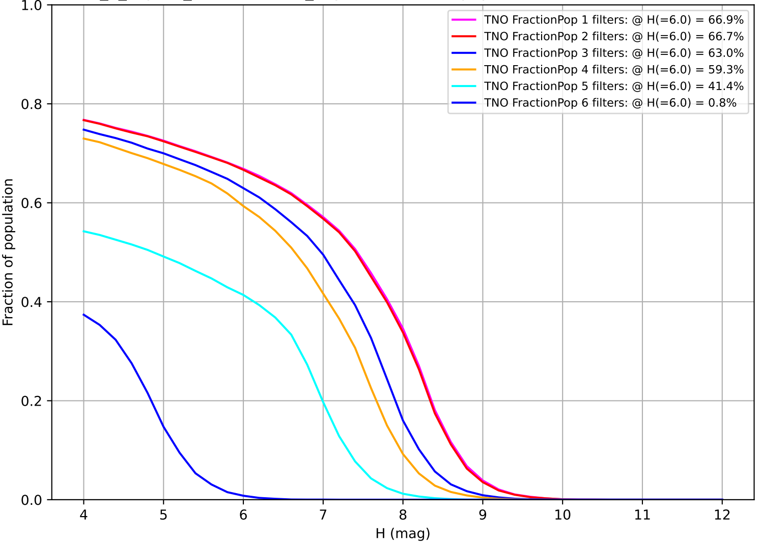
uniform_u_expt38_nscale1.1v3.4_10yrs: Fraction of population with colors in X filters TNO
