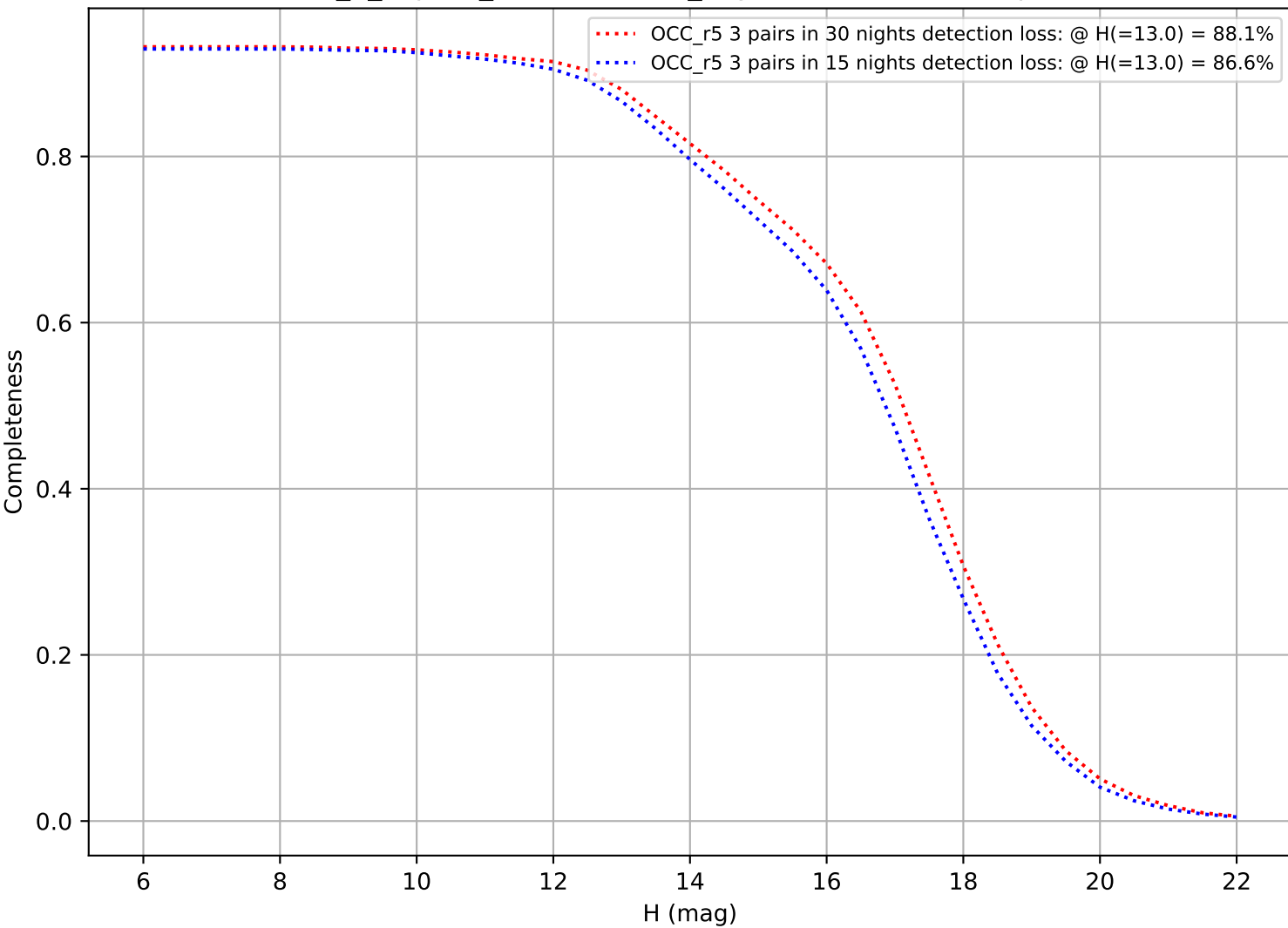
uniform_u_expt38_nscale1.1v3.4_10yrs: DifferentialCompleteness
