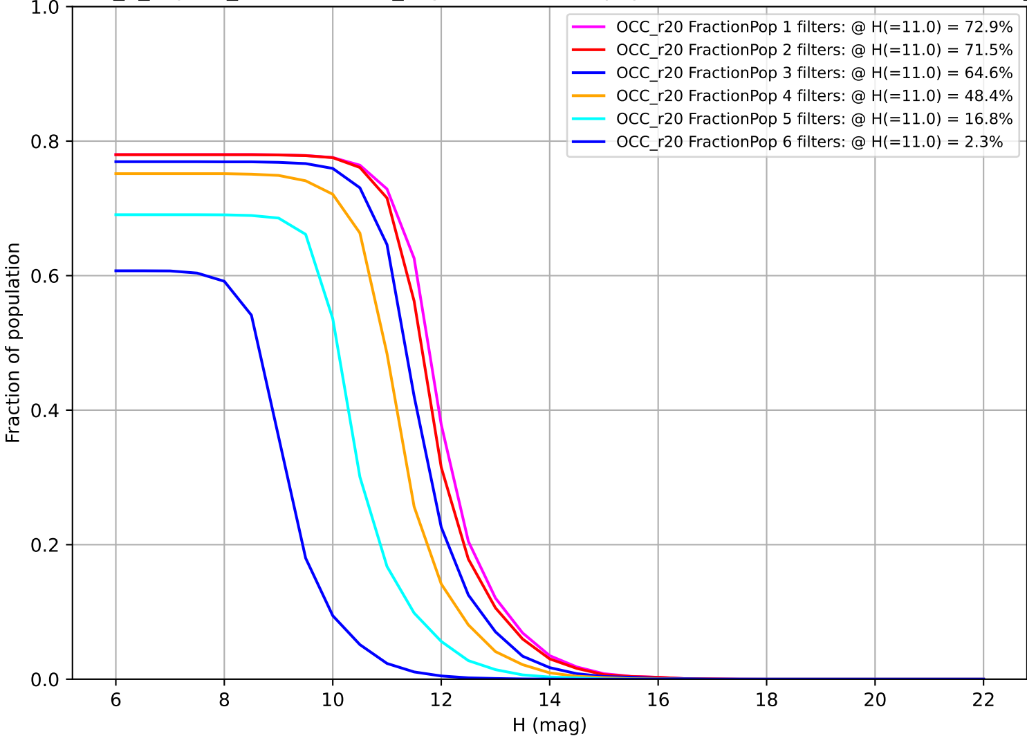
uniform_u_expt38_nscale1.1v3.4_10yrs: Fraction of population with colors in X filters OCC_r20
