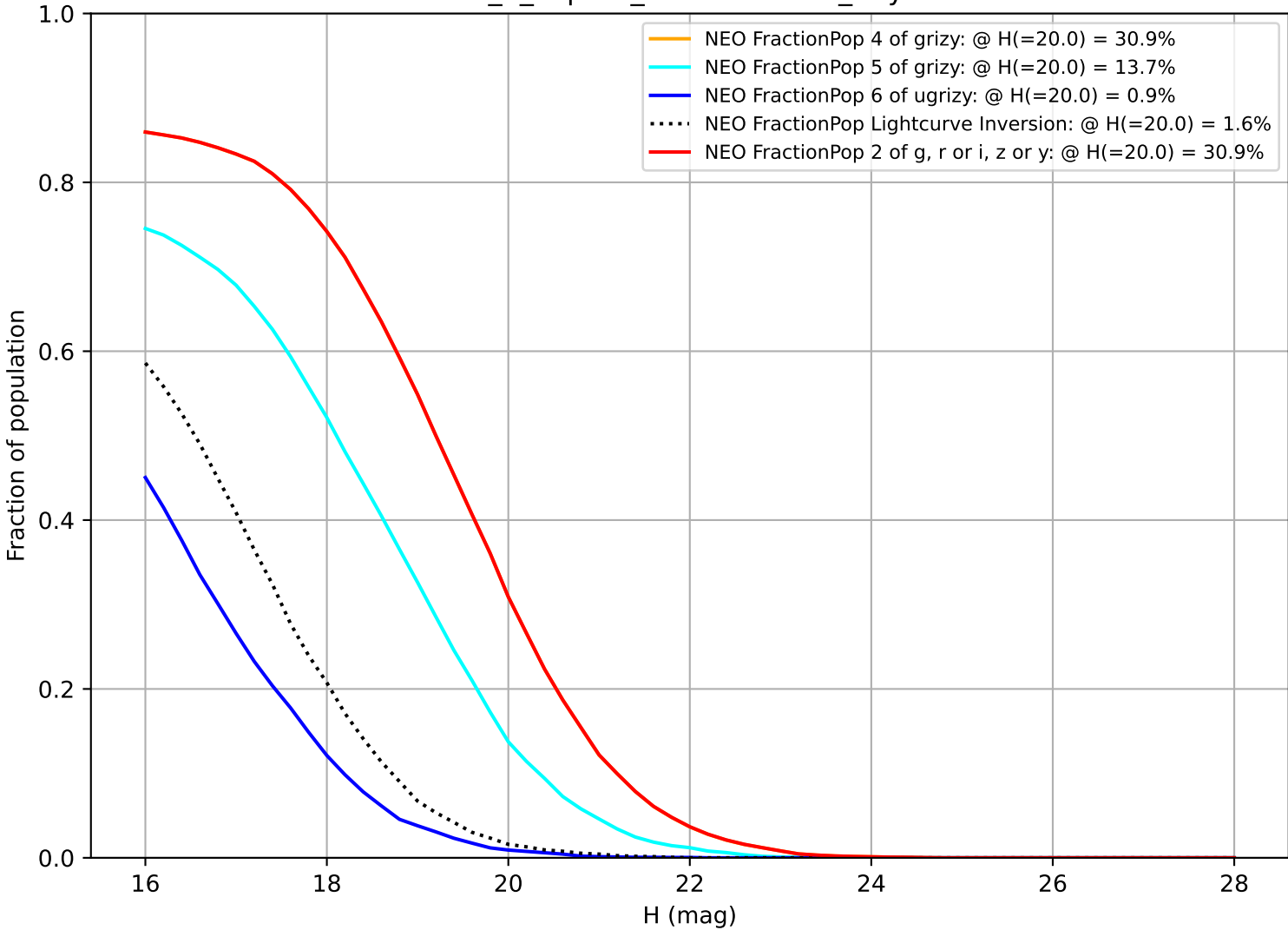
uniform_u_expt38_nscale1.1v3.4_10yrs NEO
