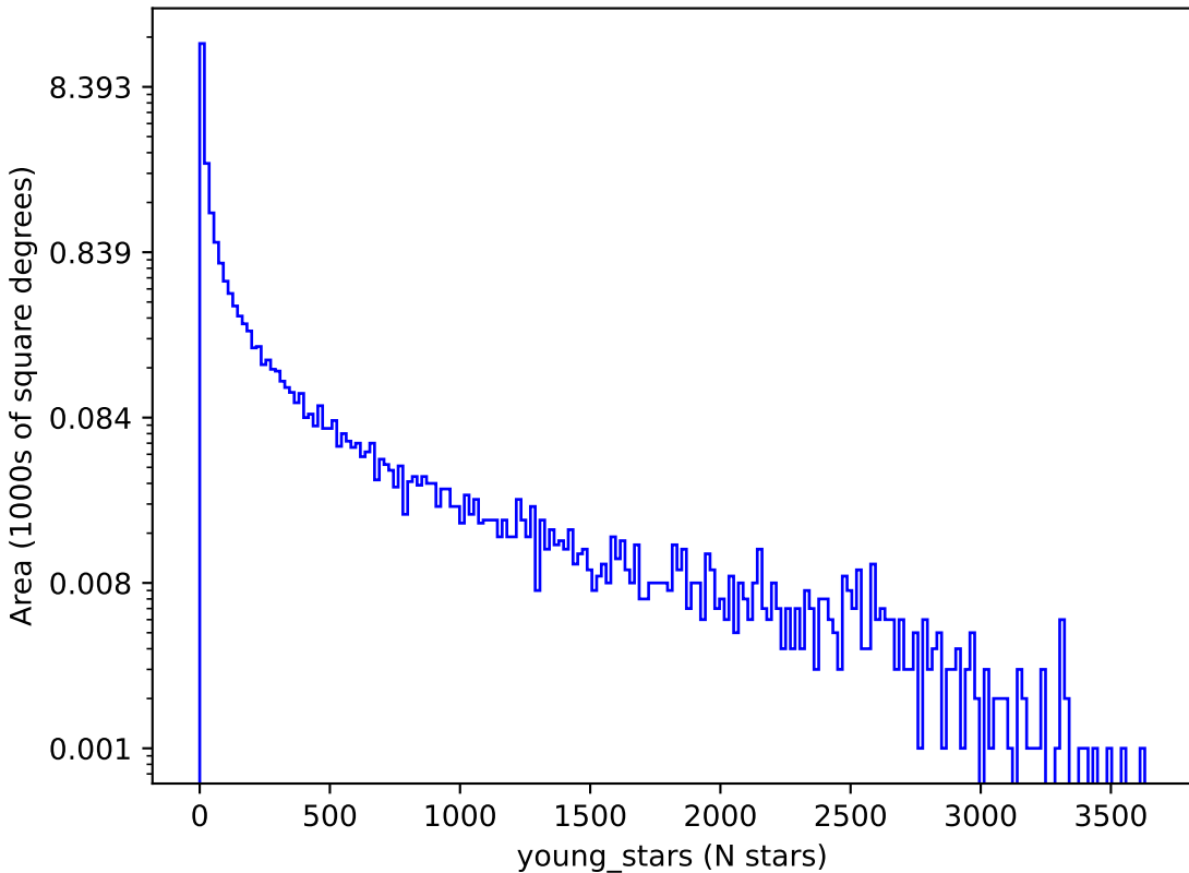
uniform_u_expt38_nscale1.1v3.4_10yrs : young_stars
