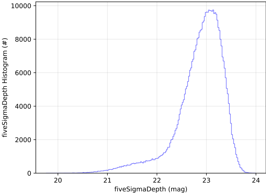
uniform_u_expt38_nscale1.1v3.4_10yrs z: fiveSigmaDepth Histogram
