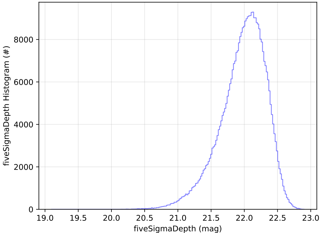
uniform_u_expt38_nscale1.1v3.4_10yrs y: fiveSigmaDepth Histogram
