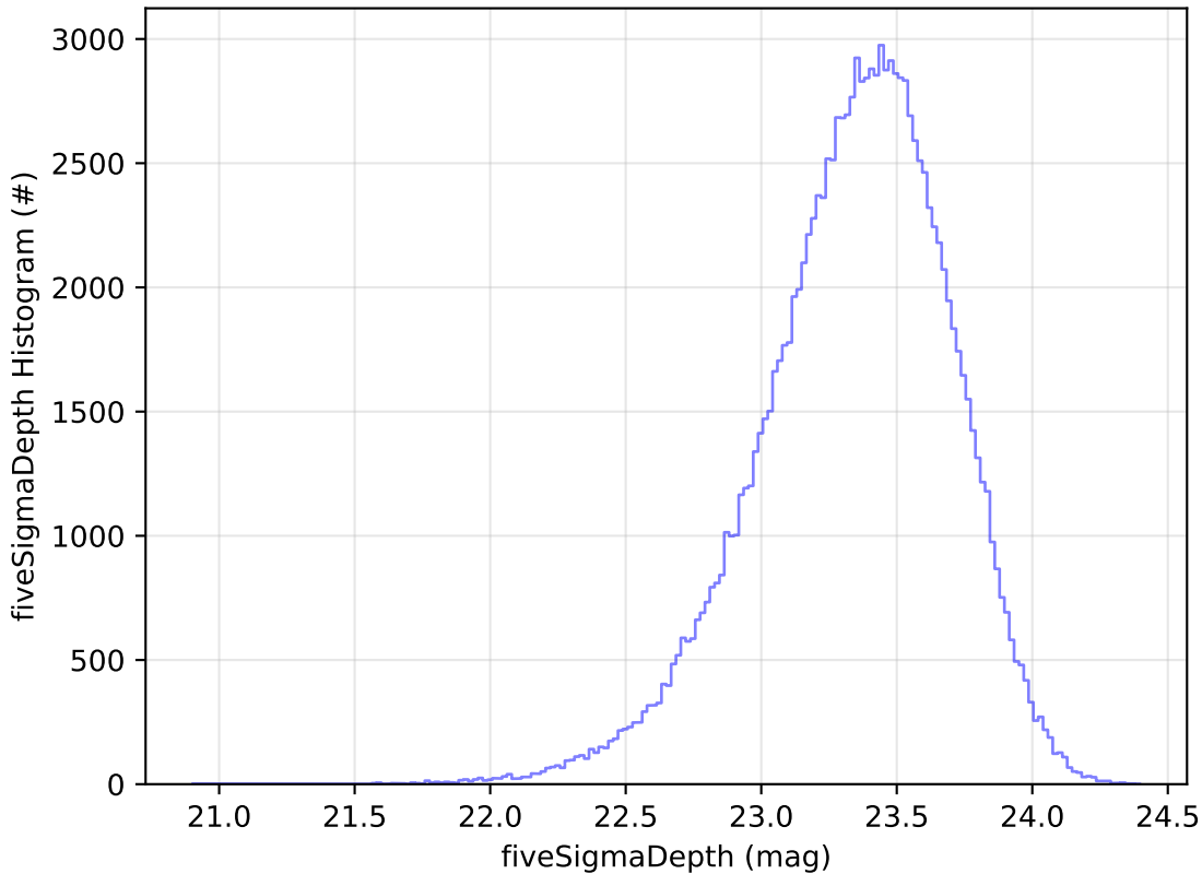
uniform_u_expt38_nscale1.1v3.4_10yrs u: fiveSigmaDepth Histogram
