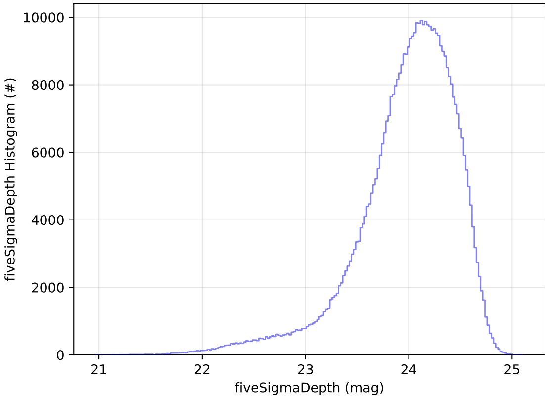
uniform_u_expt38_nscale1.1v3.4_10yrs r: fiveSigmaDepth Histogram
