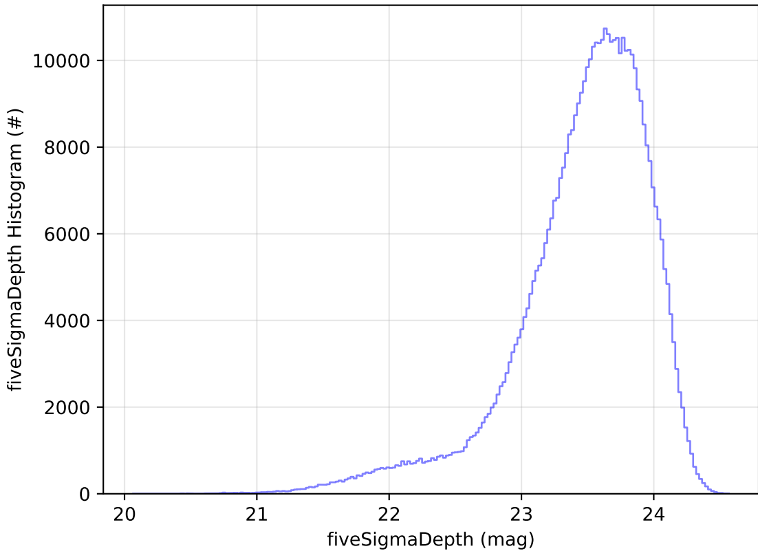
uniform_u_expt38_nscale1.1v3.4_10yrs i: fiveSigmaDepth Histogram
