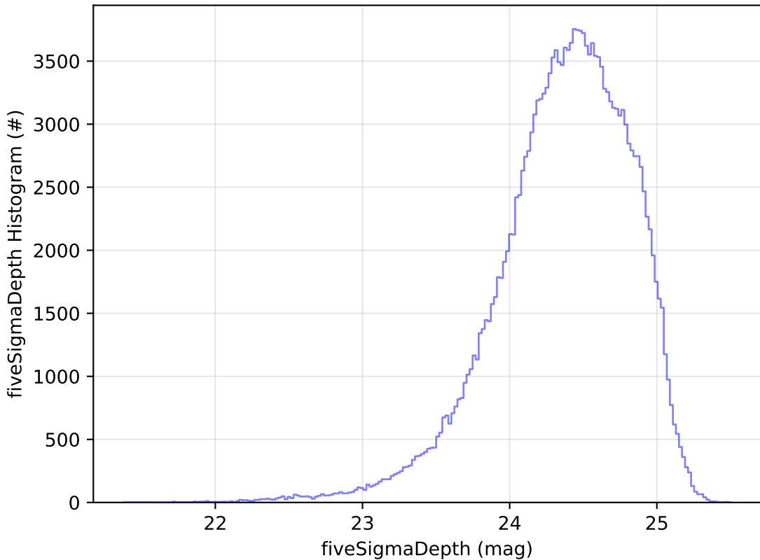
uniform_u_expt38_nscale1.1v3.4_10yrs g: fiveSigmaDepth Histogram
