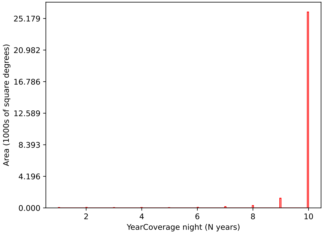
uniform_u_expt38_nscale1.1v3.4_10yrs i band: YearCoverage night
