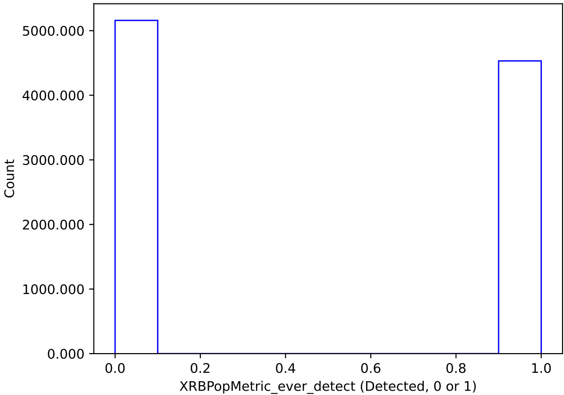
uniform_u_expt38_nscale1.1v3.4_10yrs : XRBPpopMetric_ever_detect
