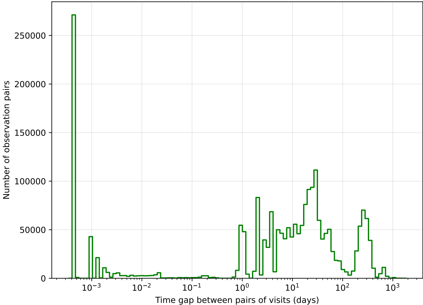
uniform_u_expt38_nscale1.1v3.4_10yrs g band: Tgaps observationStartMJD
