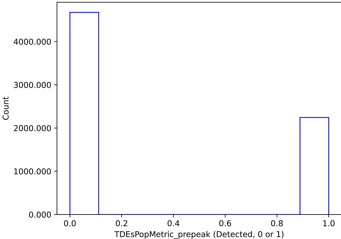
uniform_u_expt38_nscale1.1v3.4_10yrs : TDEsPopMetric_prepeak
