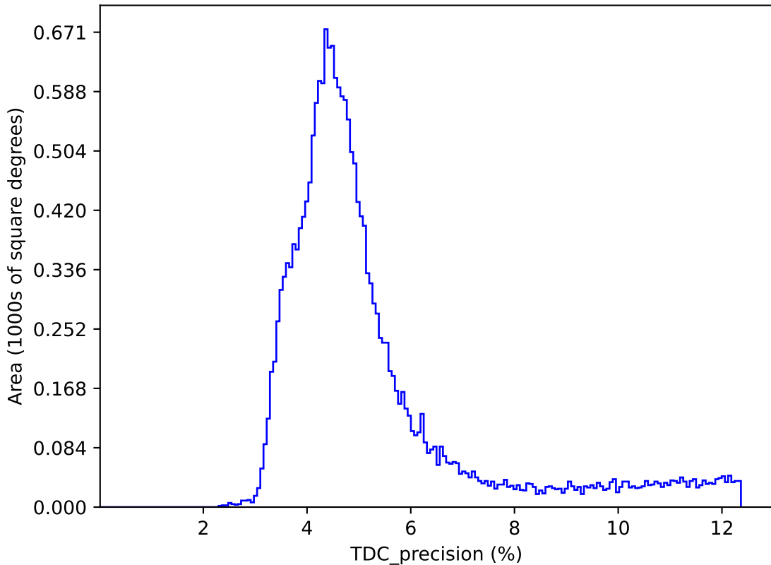
uniform_u_expt38_nscale1.1v3.4_10yrs : TDC_precision
