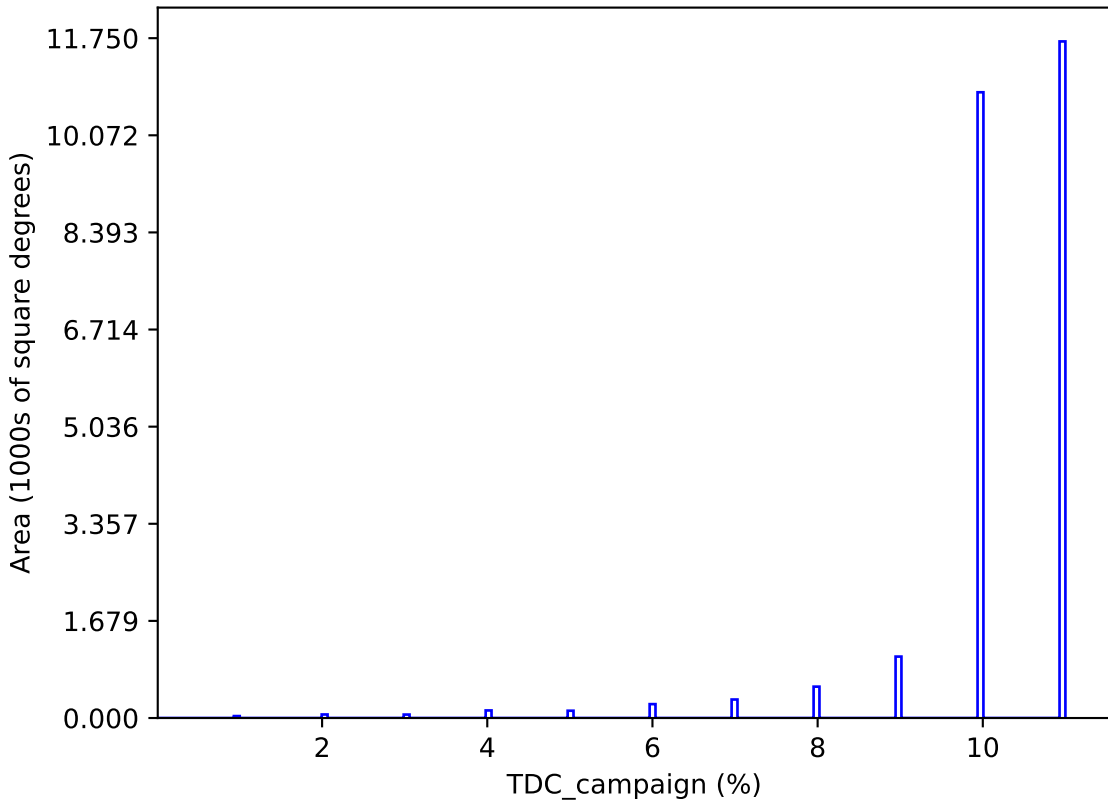
uniform_u_expt38_nscale1.1v3.4_10yrs : TDC_campaign
