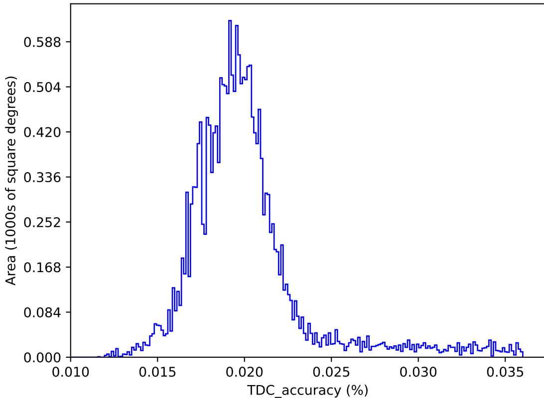
uniform_u_expt38_nscale1.1v3.4_10yrs : TDC_accuracy
