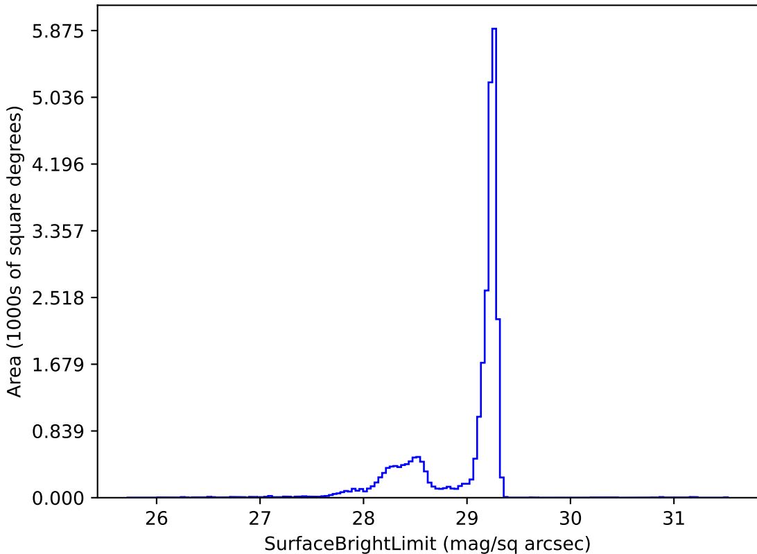
uniform_u_expt38_nscale1.1v3.4_10yrs z: SurfaceBrightLimit
