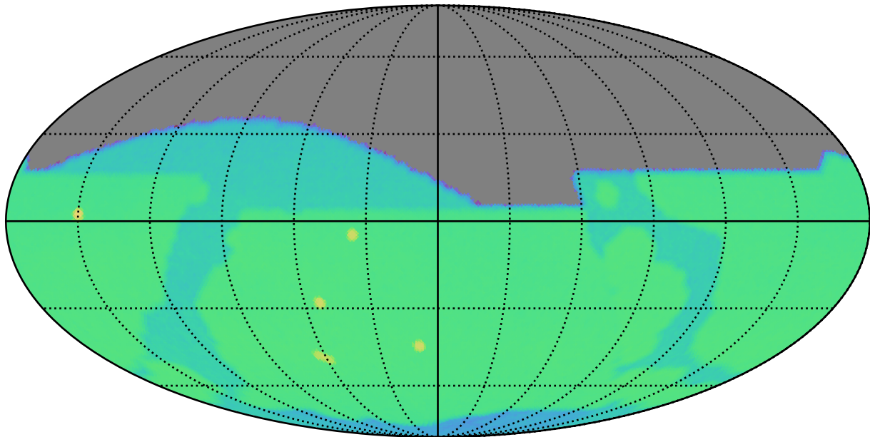
uniform_u_expt38_nscale1.1v3.4_10yrs r: SurfaceBrightLimit
