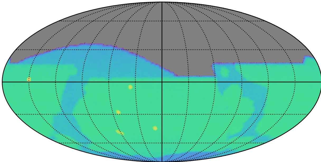
uniform_u_expt38_nscale1.1v3.4_10yrs i: SurfaceBrightLimit
