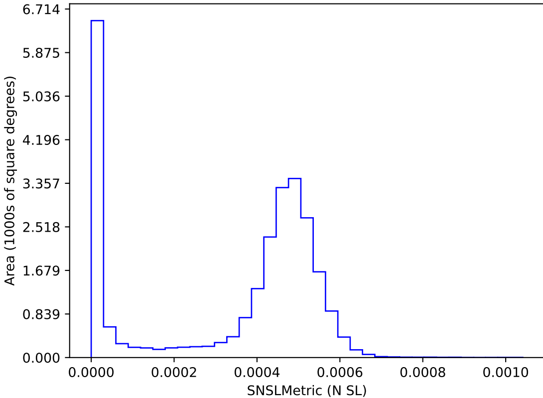
uniform_u_expt38_nscale1.1v3.4_10yrs : SNSLMetric
