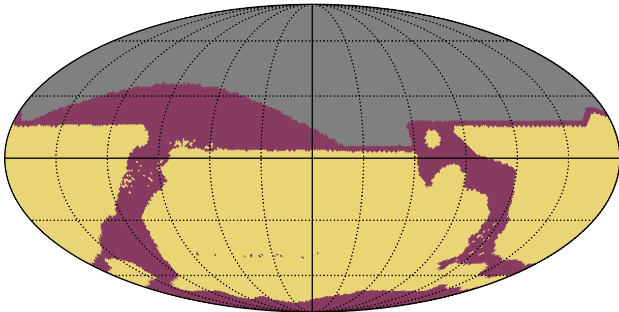
uniform_u_expt38_nscale1.1v3.4_10yrs : RapidRevisits
