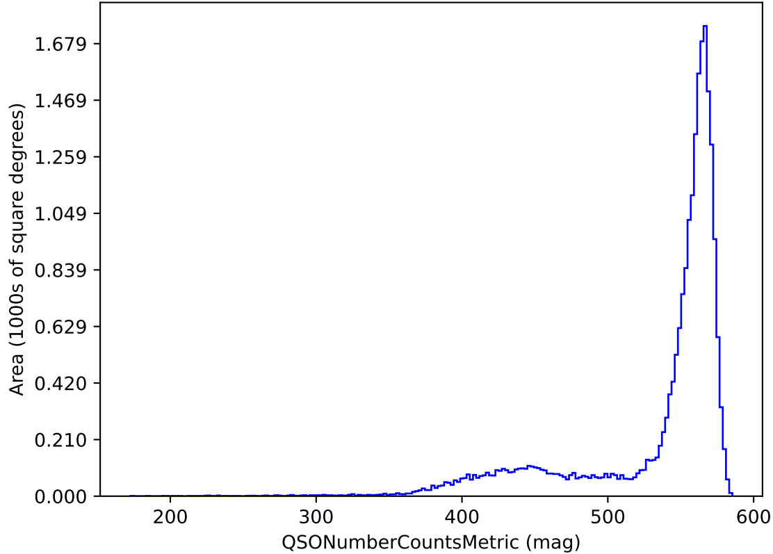
uniform_u_expt38_nscale1.1v3.4_10yrs y band and non-DD: QSONumberCountsMetric
