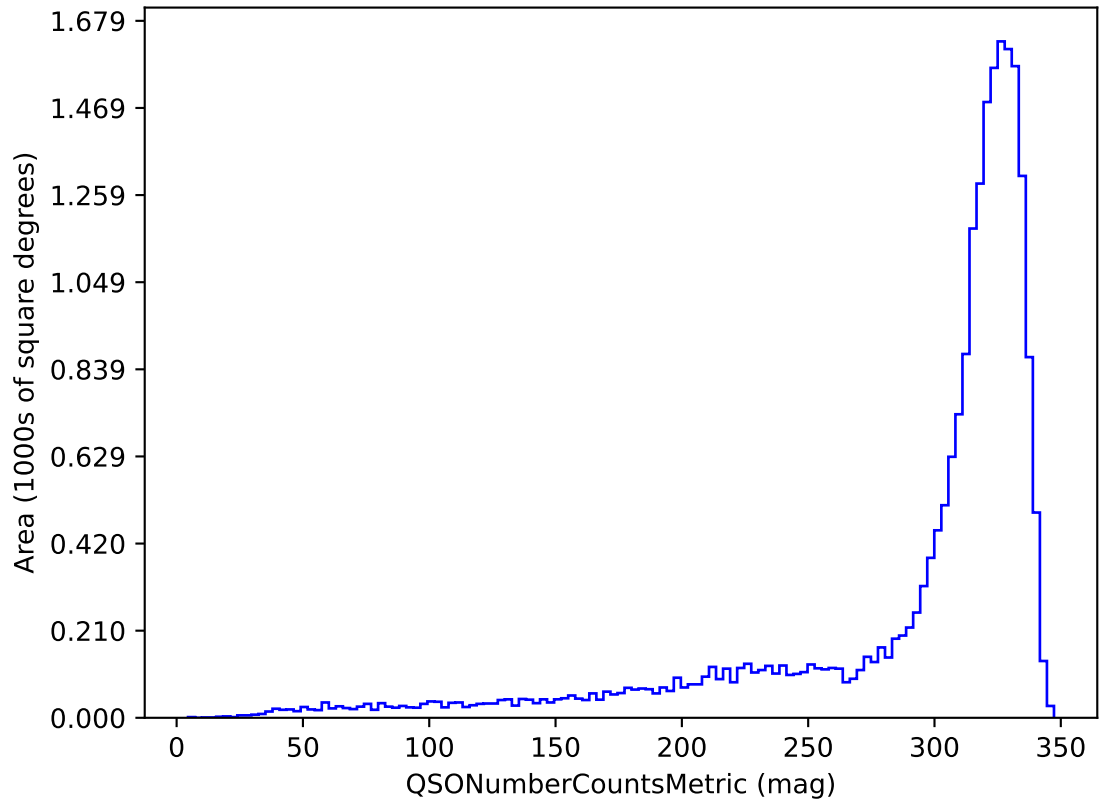
uniform_u_expt38_nscale1.1v3.4_10yrs u band and non-DD: QSONumberCountsMetric
