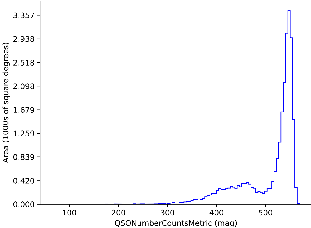
uniform_u_expt38_nscale1.1v3.4_10yrs i band and non-DD: QSONumberCountsMetric
